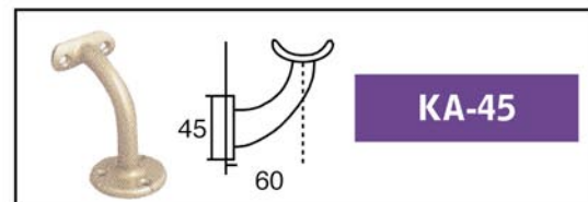
Infinity Standard Handrail - Ø 45mm
