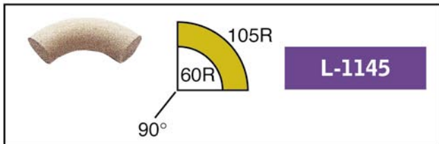
Infinity Standard Handrail - Ø 45mm
